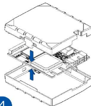
Attaching cover back
