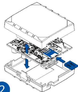
Micro-SIM card insert
