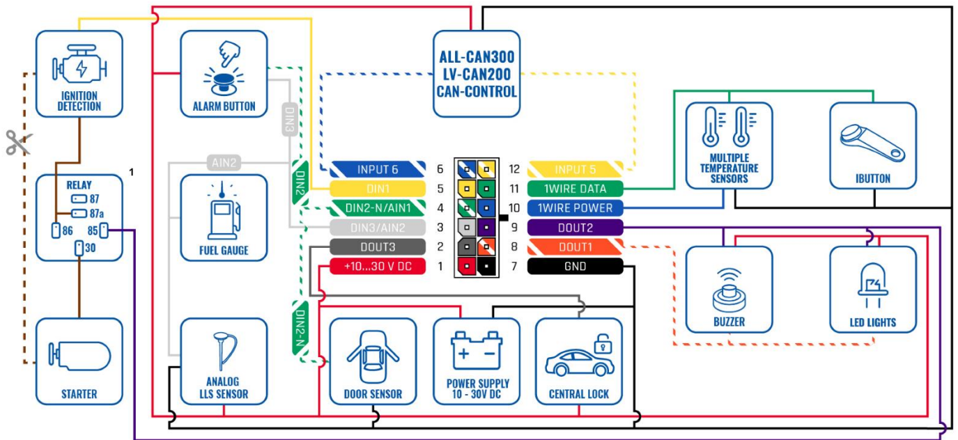
ACT 300 Wiring scheme
